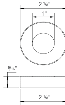
Optional Flange Cover
