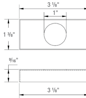
Optional Flange Cover
