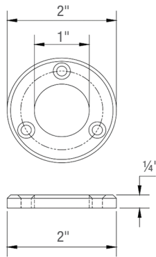
Mounting Flange
