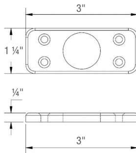
Mounting Flange
